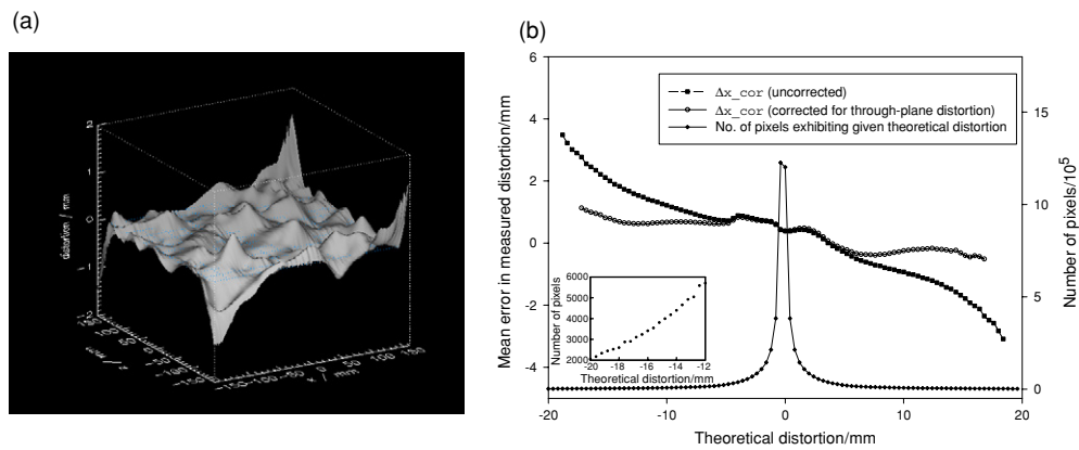
Figure 6. Illustration of the correction of distortion maps for through-plane distortion. (a) Coronal view of the correction to the x -distortion map, showing significant values at the corners of the region of support. (b) Left-hand axis: mean error in the measured x -distortion for all pixels with a given theoretical x -distortion. This plot shows that the errors are not random, but due to the phenomenon of slice warp. The correction applied is successful reducing the mean error well below 1 voxel-width. Right-hand axis: illustration of the significance of the distortion problem in terms of numbers of pixels affected, with (inset) an enlargement for the region of high distortion. The binsize for these histograms is 0.4 mm.
