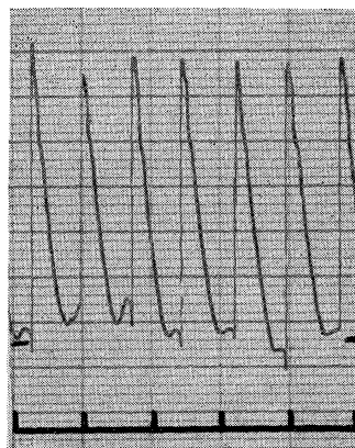
FIG. 7. Photograph of the central portion of a steady-state free precession response from an oxygen-free water sample with T_1 \doteq 3.5 sec. The effect of a sweep time comparable to the relaxation time is illustrated. Time increases to the left. Each marker indicates 10 sec.
